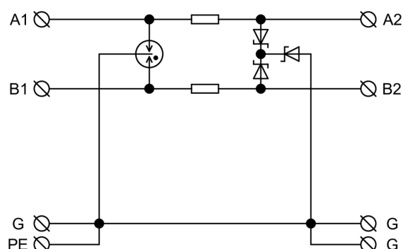
Internal diagram
